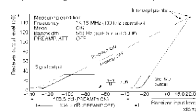
• Dynamic range characteristics example
