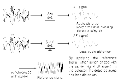
• Difference between AM and S-AM detection
