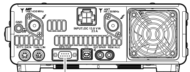
Prise jack GPS/CAT
