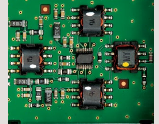
Mixer Unit
