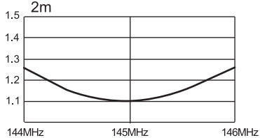
V.SWR chart (X-50N)
